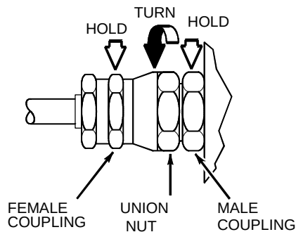
DISCONNECTING FROM COMPRESSOR
